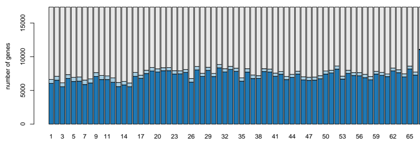
Figure 2: Present/absent calls. The barplot shows, for each of the 66 arrays, the number of genes targeted by probe sets with "A" (light grey), "M" (light blue) and "P" (blue) calls. The 67-th bar at the very right corresponds to detection in at least 10% of arrays.
